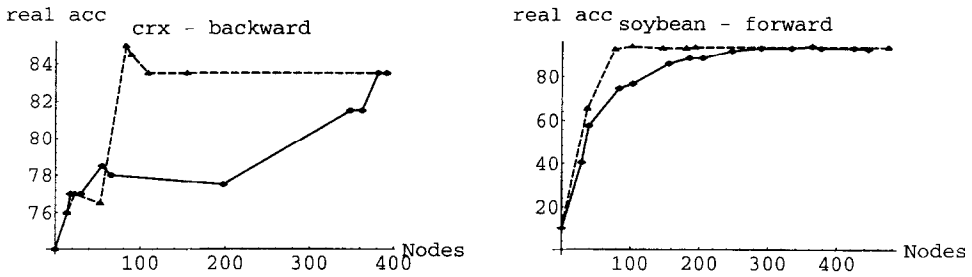
Fig. 15. Comparison of compound (dotted line) and non-compound (solid line) searches. The accuracy ( y -axis) is that of the best node (as determined by the algorithm) on an independent test set after a given number of node evaluations ( x -axis). The running time is proportional to the number of nodes evaluated.
